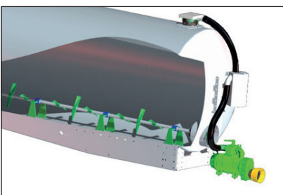
Integrated mixer with direct connection to the tractor (option).
