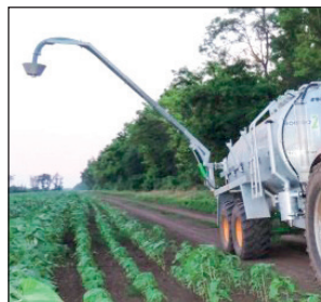
Rotation and lifting through hydraulic rams.
