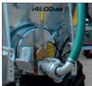
Connection to the valve and quick coupling of the scatterer.
